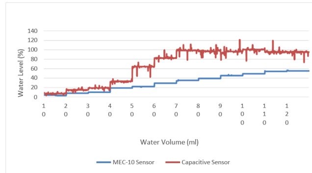
Fig. 2. Water level in planting media (for experiment using 120 ml water)
